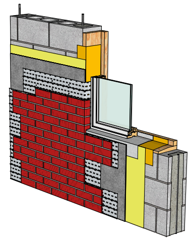
05. Pan flashing
