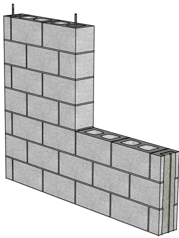
01. Concrete masonry backing
