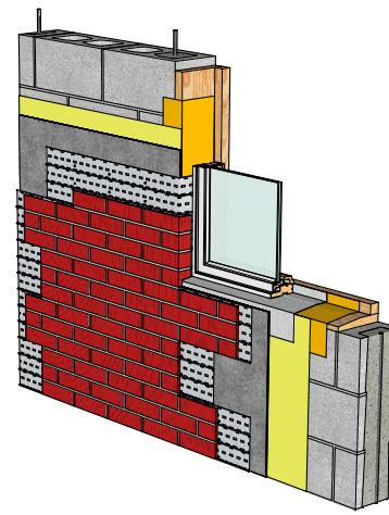
04. Air barrier
