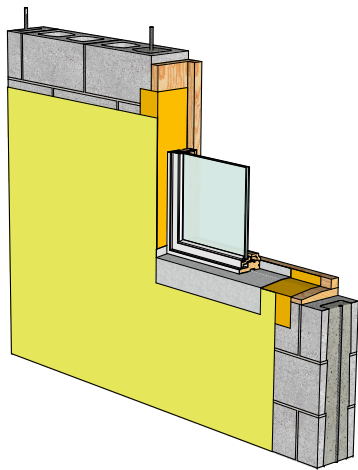
06. Window assembly
