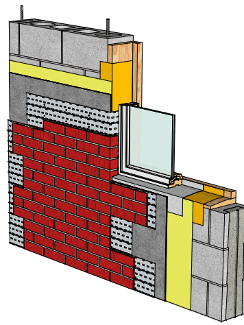
03. Transition membrane
