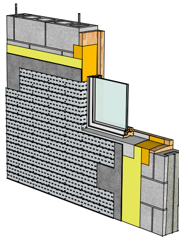
08. Patented grid panel
