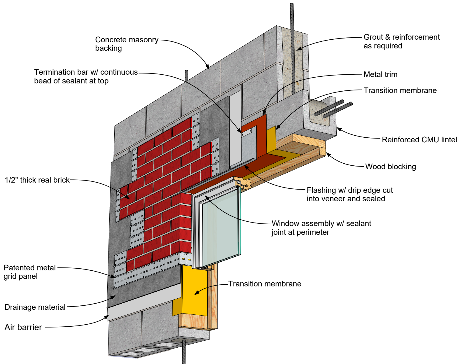
MCS Exterior Wall, CMU Backing | Window Head Detail 03.01.03 Rev. 02/10/19
