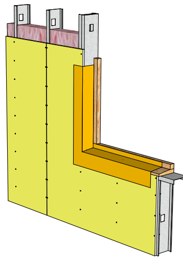
03. Transition membrane
