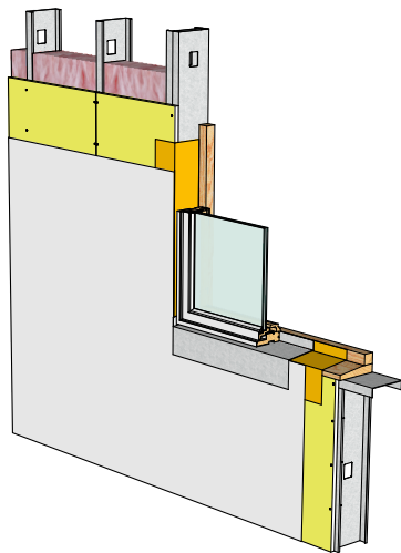
06. Window assembly
