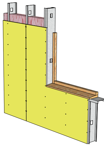
02. Wood blocking
