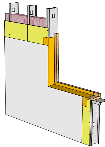
04. Air barrier
