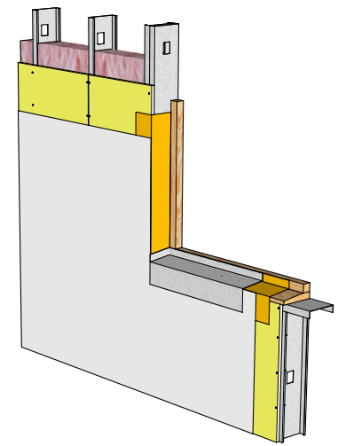
05. Pan flashing
