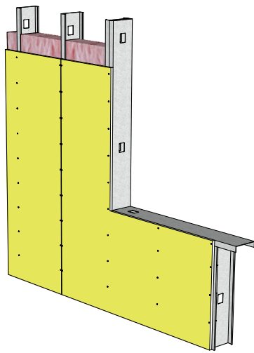
01. Steel studs, sheathing, insul.
