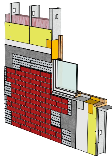
09. Real thin brick
