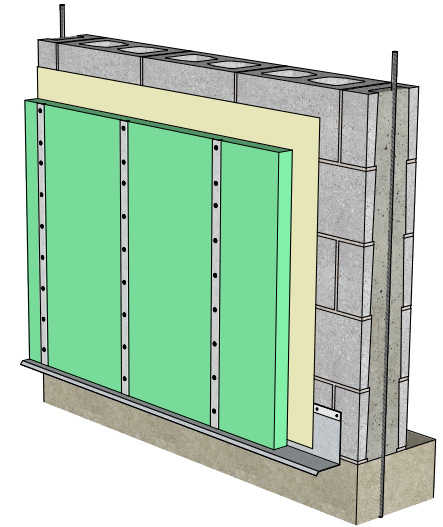
04. Insulation
