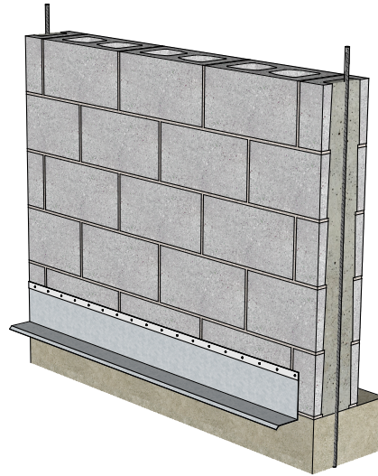
02. Flashing
