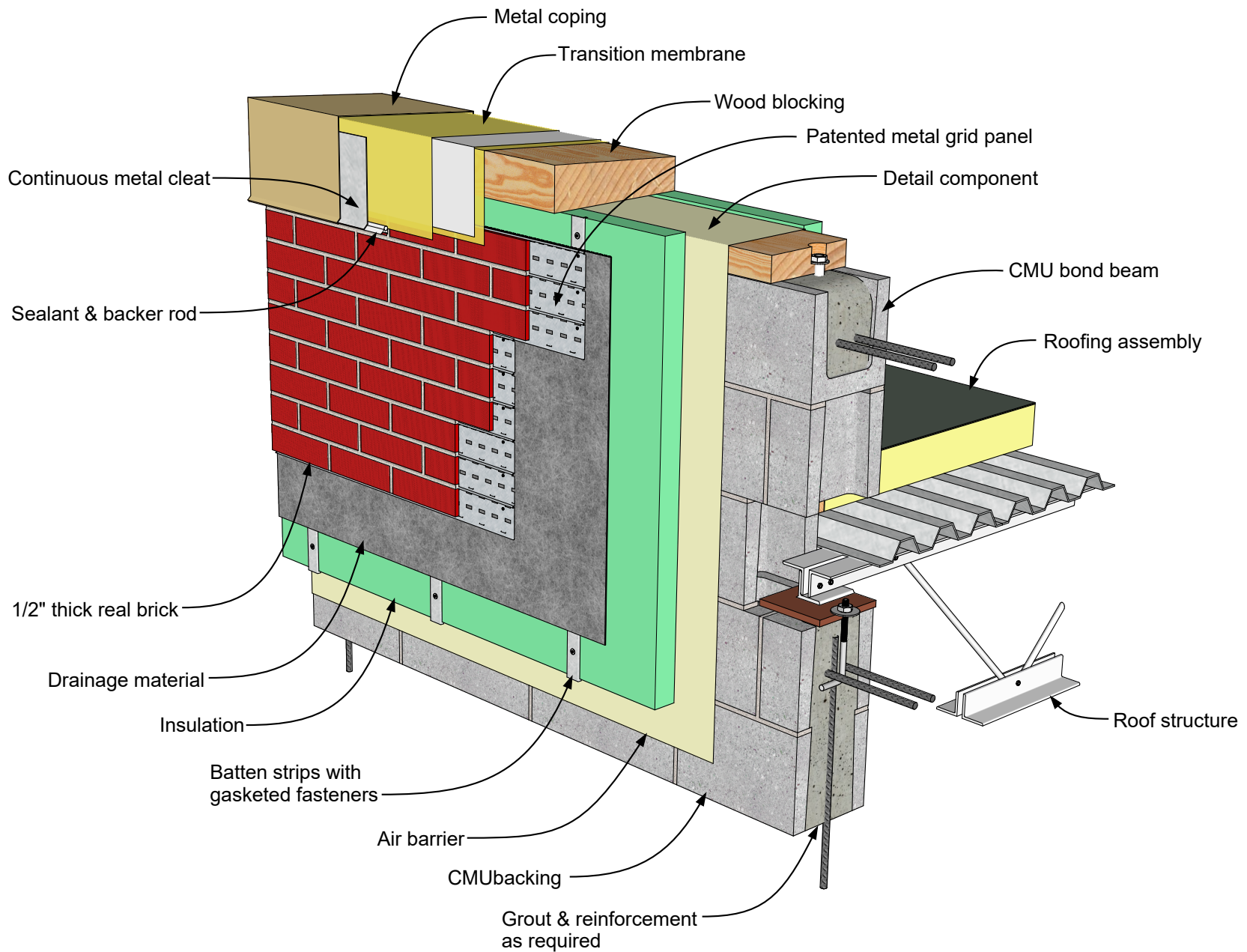
CIS Exterior Wall, CMU Backing | Top of Wall Detail 05.01.06 Rev. 12/28/18
