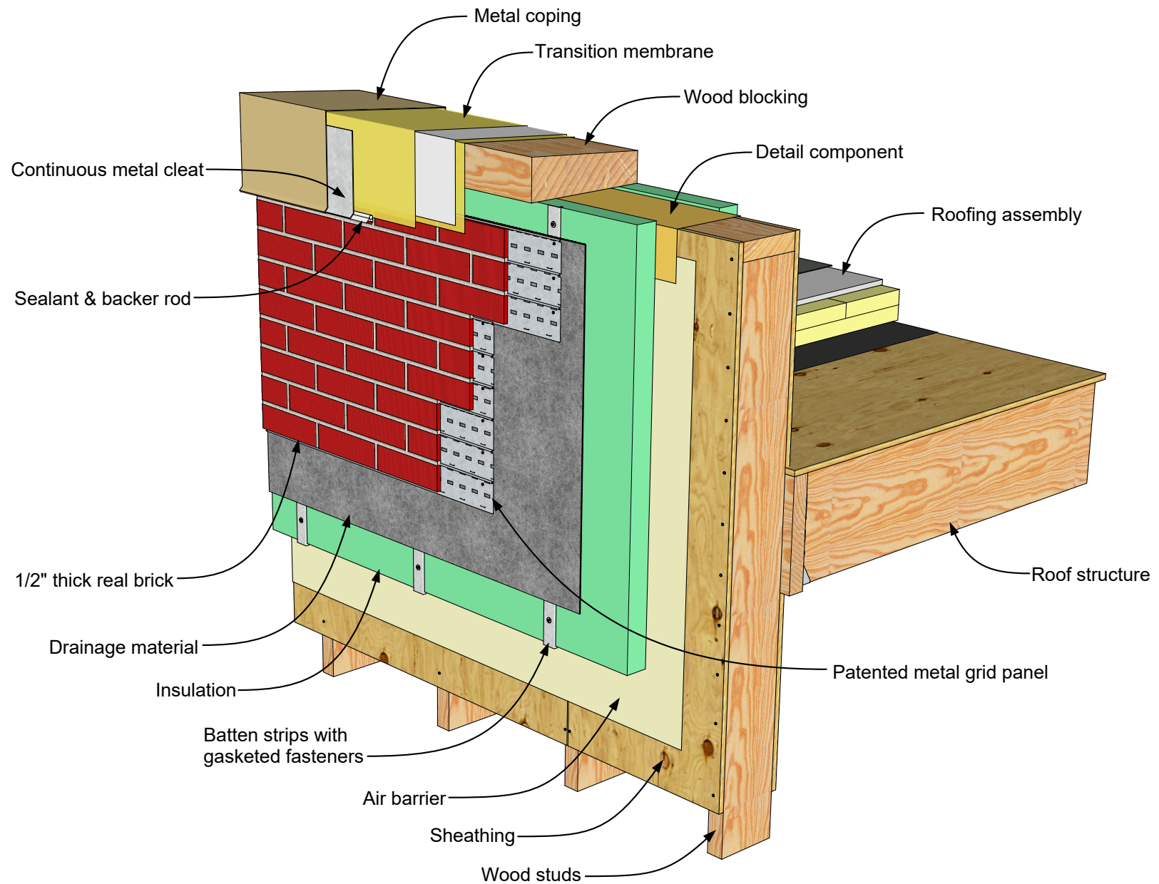
CIS Exterior Wall, Wood Stud Backing | Top of Wall Detail 05.02.06 Rev. 12/16/18
