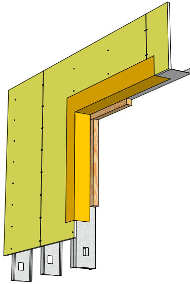
02. Transition membrane
