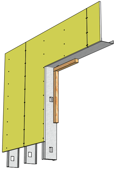
01. Studs, sheathing, blocking
