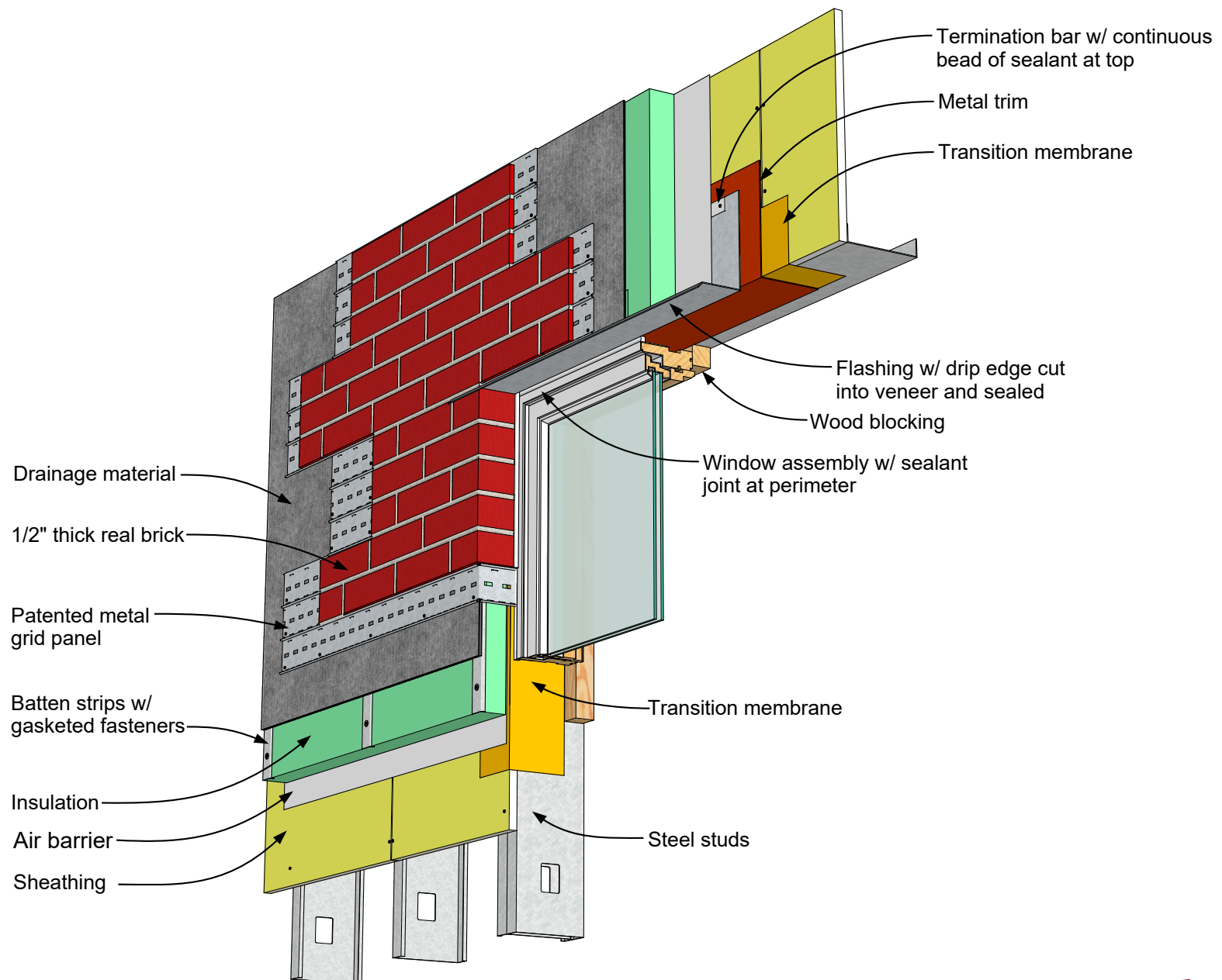
CIS Exterior Wall, Steel Stud Backing | Window Head Detail 05.03.03 Rev. 12/26/18
