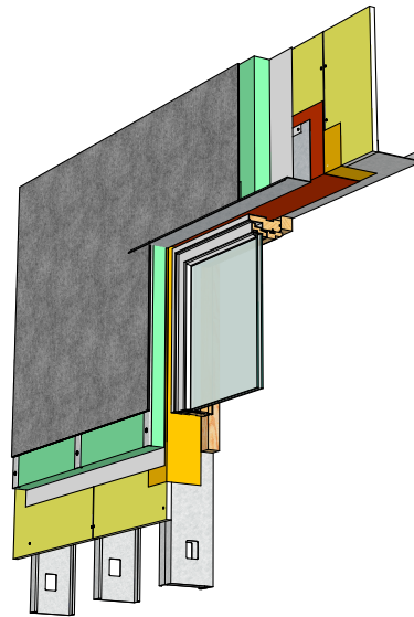
08. Drainage material
