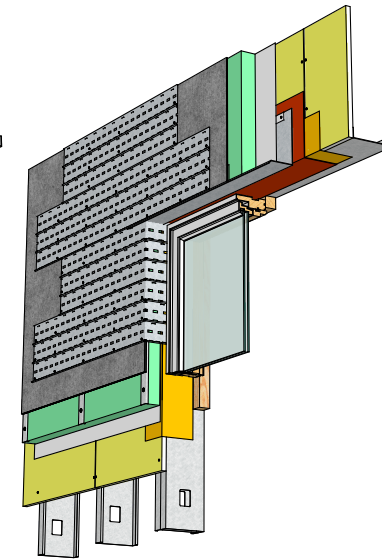
09. Patented grid panel
