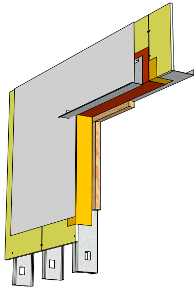
06. Air barrier
