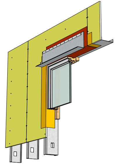
05. Pan flashing & term. bar
