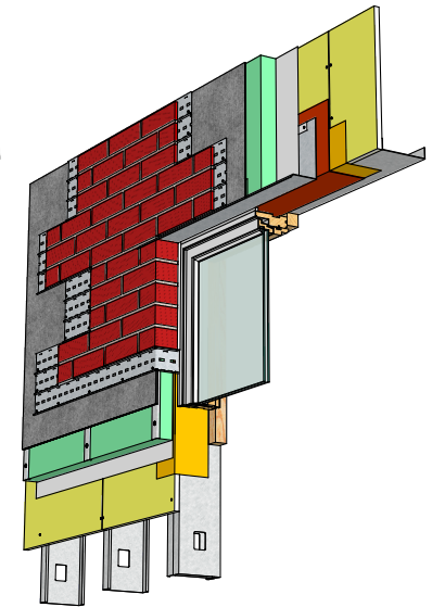
10. Real thin brick
